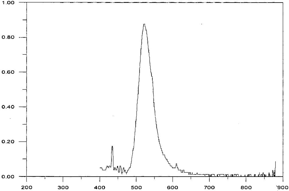
Spectrum of Green Electroluminescent Layer
